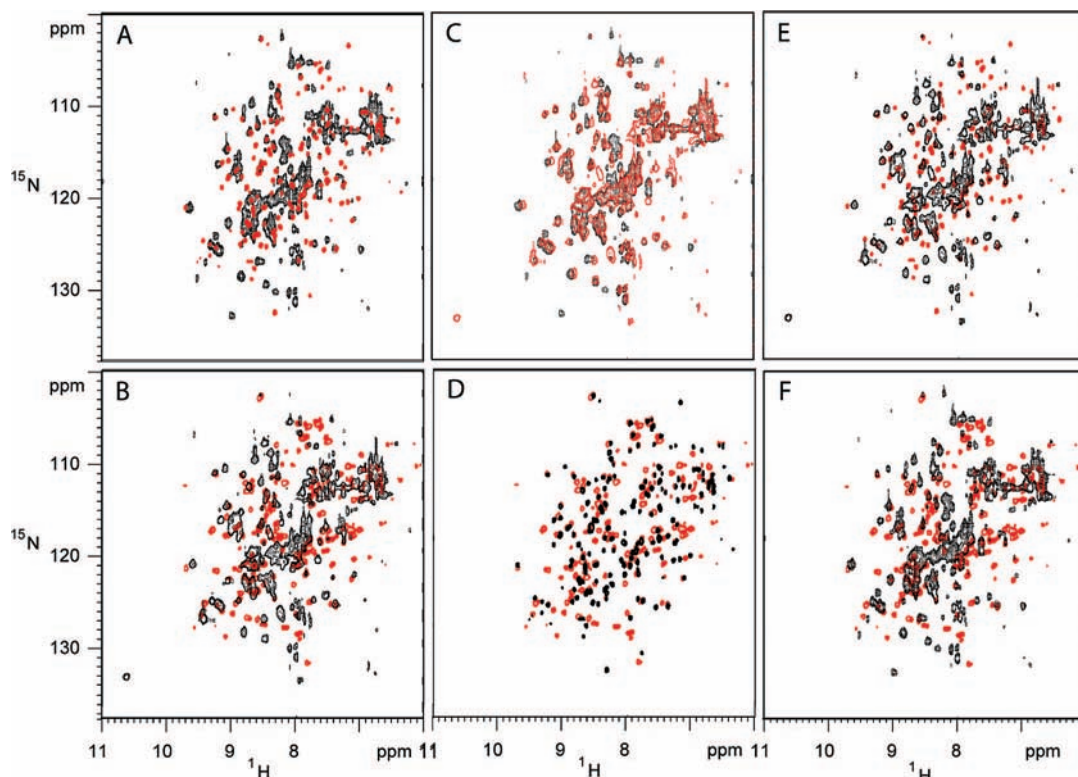
Figure 4. Superimposition of the spectra of (A) apoHasA (red) with apoHasA–HasR (black), (B) holoHasA (red) with holoHasA–HasR (black), (C) apoHasA–HasR (black) with holoHasA–HasR (red), (D) apoHasA (black) with holoHasA (red), (E) apoHasA (red) with holoHasA–HasR (black), and (F) holoHasA (red) with apoHasA–HasR (black).
