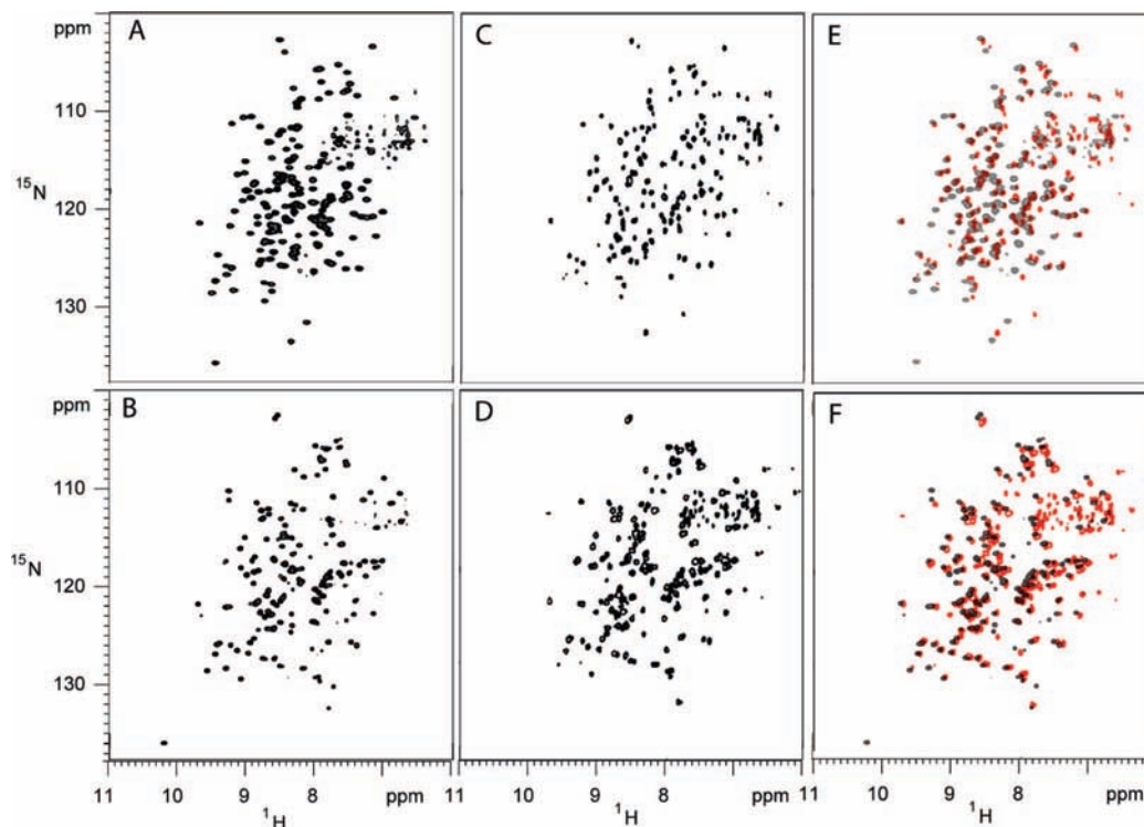
Figure 2. Comparison of the NMR spectra obtained for ( ^2\text{H} , ^{15}\text{N} ) apoHasA and holoHasA under different experimental conditions: 500 MHz TROSY spectra of (A) 1.2 mM apoHasA and (B) 1 mM holoHasA, both in 20 mM phosphate buffer pH 7; 900 MHz TROSY spectra of (C) 0.4 mM apoHasA and (D) 0.4 mM holoHasA, both in 5 mM DPC and 20 mM phosphate buffer pH 7; (E) superimposition of the apoHasA spectra reported in panels A (black) and C (red) and (F) superimposition of the holoHasA spectra reported in panels B (black) and D (red).
