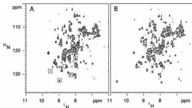
Figure 3. CRINEPT–TROSY spectra of (A) apoHasA–HasR and (B) holoHasA–HasR acquired at 900 MHz, in 5 mM DPC and 20 mM phosphate buffer pH 7. Protein concentrations were 320 \mu\text{M} for apoHasA–HasR and 360 \mu\text{M} for holoHasA–HasR. Boxed peaks in panel A are not present in the spectrum of holoHasA–HasR. A possible candidate peak for Tyr75 in panel B is labeled with a red star.
